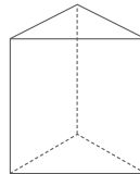
Prisma triangular
